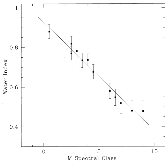
FIG. 3.—Plot of the water vapor index Q vs. MV subclass for our M dwarf standards. Spectral types were adopted from Kirkpatrick et al. (1991). Error bars reflect 1\sigma uncertainties in Q from the statistical uncertainties in calculating F1, F2, and F3. The solid line is the best fit to the data (eq. [2]).
