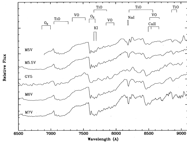
FIG. 5.—An optical spectrum for the brown dwarf candidate GY 5 relative to dwarf spectral standards of Kirkpatrick et al. (1991). The spectrum of this PMS object appears intermediate to that of a M5.5 and M6 dwarf. Labeled on the plot are photospheric atomic absorptions due to K I, Na I, and Ca II and molecular absorptions from TiO and VO. Features labeled as O 2 are telluric in nature. For a more complete identification of features, see Kirkpatrick et al. (1991), Fig. 5c.
