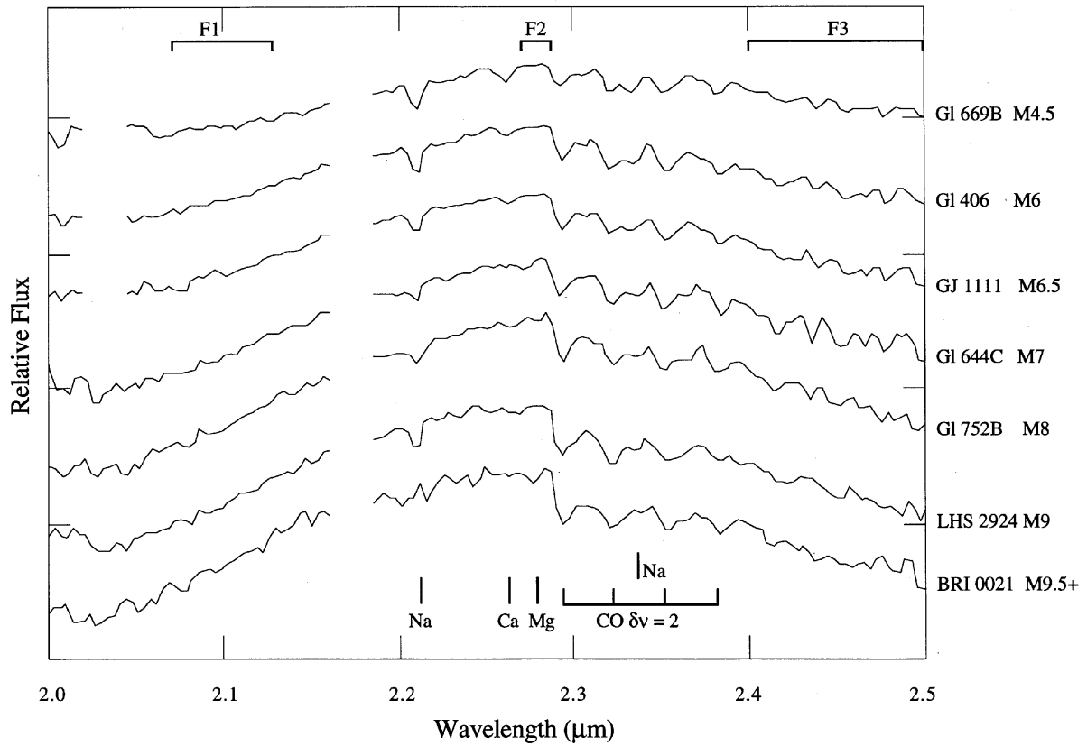
FIG. 2.—Infrared spectra of M dwarf standards at R = 300 . Spectral types were adopted from Kirkpatrick et al. (1991) or Henry et al. (1994). Top : The 2.0–2.5 \mu\text{m} spectra for dwarfs from K5 to M4; bottom : the spectra for dwarfs of spectral type M4.5 to later than M9.5. The wavelengths of absorption lines of Na, Ca, Mg, and CO are marked at the bottom of each plot. The wavelength ranges averaged to compute the water vapor index Q are labeled as F1, F2, and F3.
