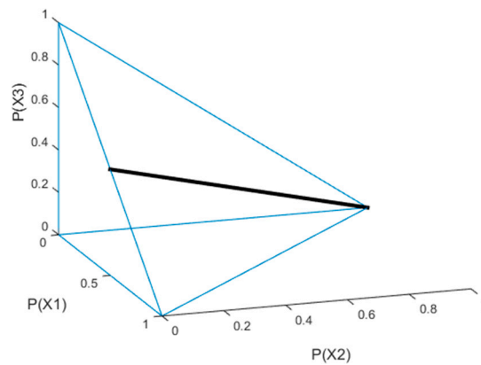
Figure 2. Feasible set (bold line) when the random variable has three outcomes.
