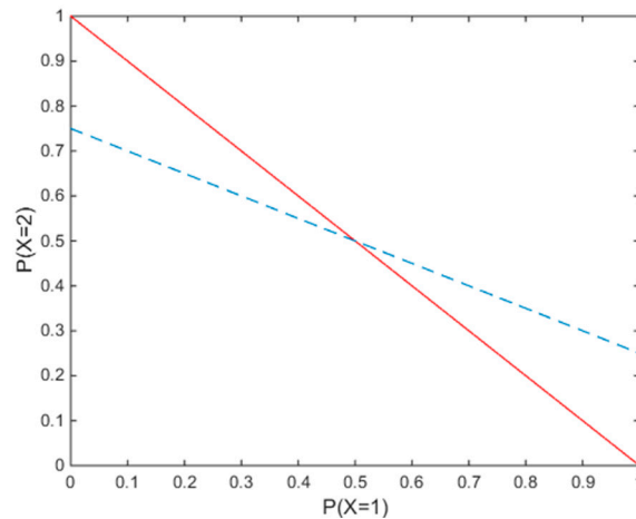
Figure 1. Feasible set for the probability distribution when the variable has two outcomes.
