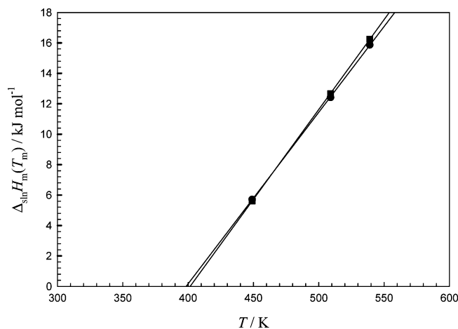
Figure 2. Effect of temperature on the magnitude of \Delta_{\text{sln}}H_{\text{m}}(T/\text{K}) . ■, eicosane; ●, nonadecane.
